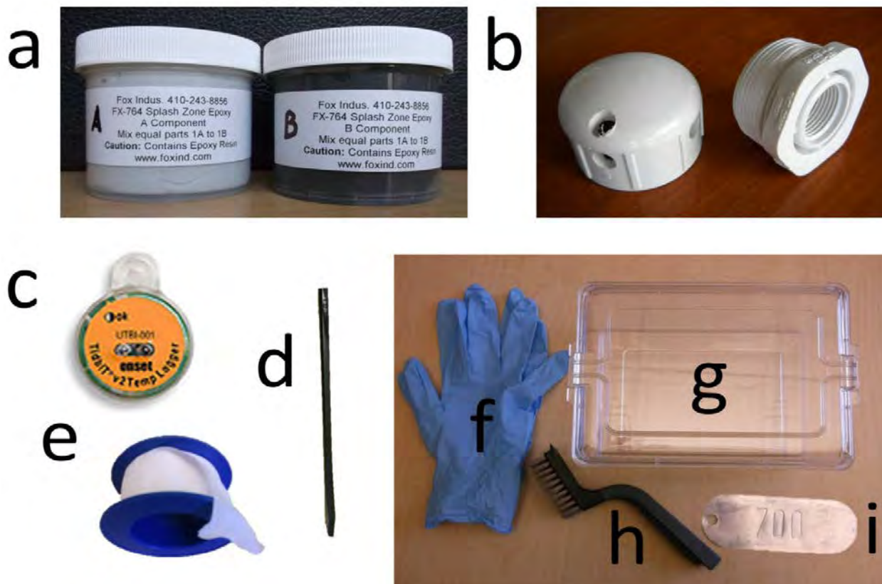
Figure 9. Equipment needed to permanently install temperature sensors in streams using underwater epoxy. The equipment includes: (a) two-part FX-764 epoxy from Fox Industries, (b) PVC solar shield, (c) temperature sensor, (d) cable ties, (e) plumber's tape, (f) rubber gloves, (g) plastic viewing box, (h) wire brush, and (i) metal forestry tree tag (Isaak and Horan 2013).
