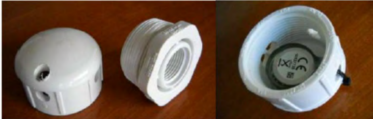
Figure 4. Unassembled components of an inexpensive PVC canister radiation shield for water temperature sensors (described in more detail in Isaak et al. 2013).
