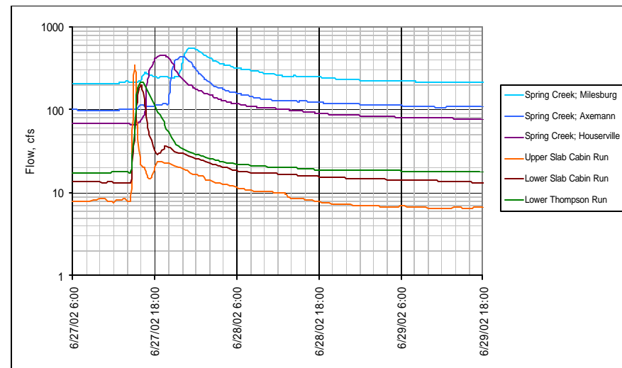
Figure 8. Storm Response in Spring Creek and Urban Tributaries.
